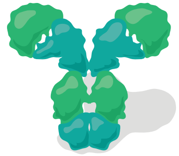
Antibody
