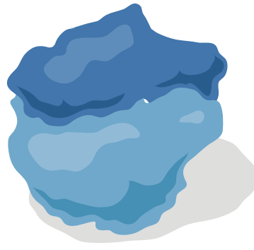
Ribosome
