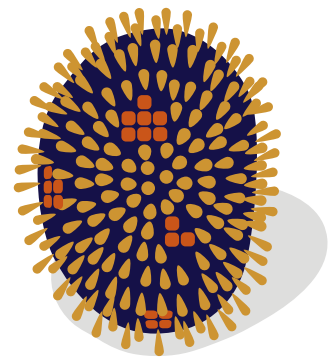
Influenza virus
